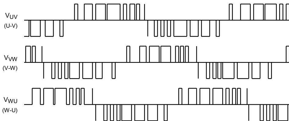
Inter-line voltage
