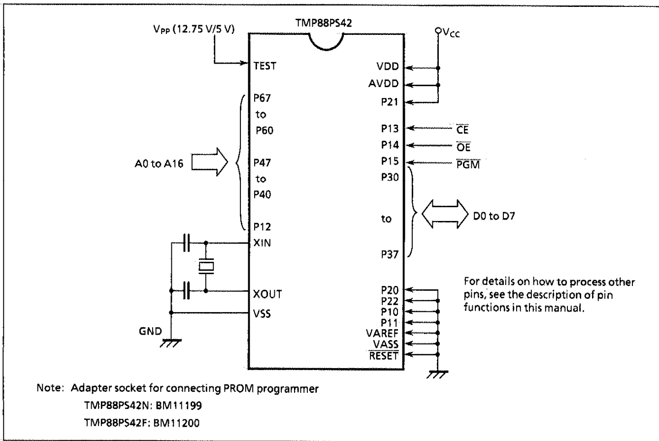
Figure 1-2. Setting Up PROM Mode
