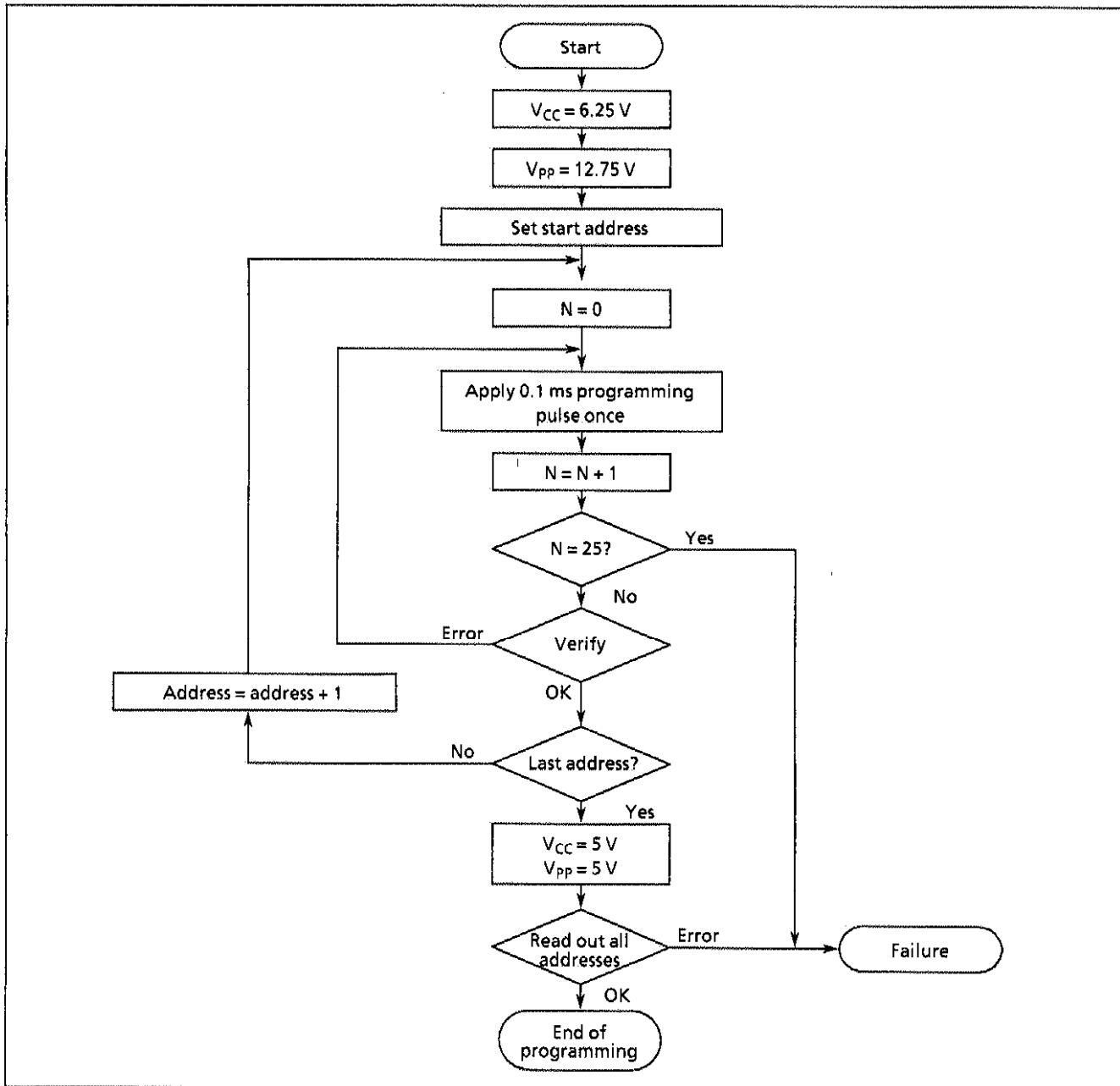
Figure 1-3. Programming Flowchart
