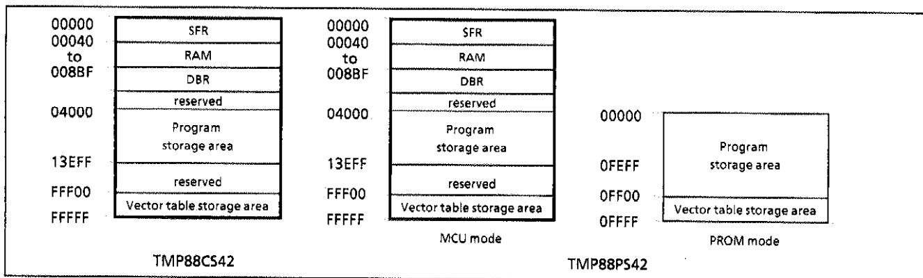
Figure 1-1. Program Storage Area
